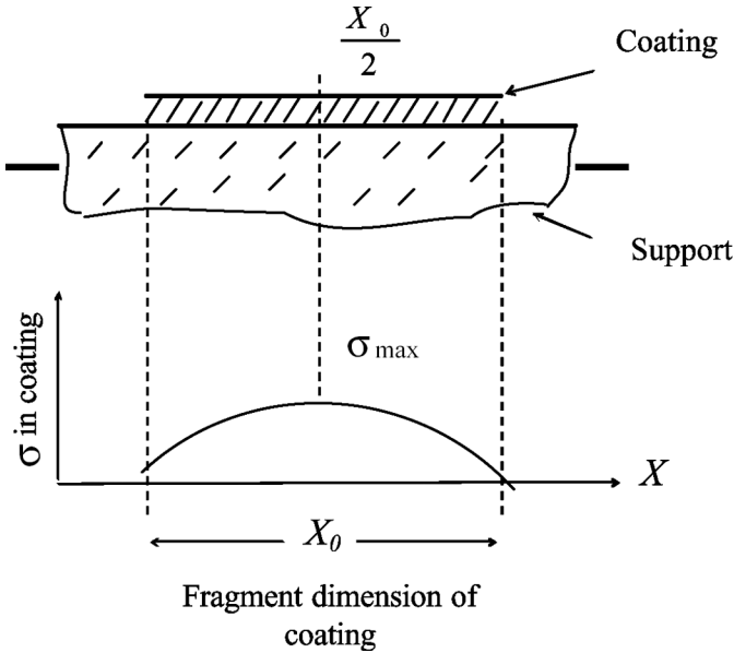
Figure 3. Schematic representation of stress distribution in a fragment of the coating during tensile drawing of the polymer substrate. X_0 is the size of the fragment. Arrows show the direction of stretching.
