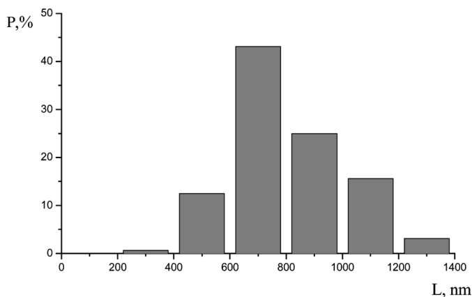
Figure 4. Fragment width distribution curve for PET films with a gold coating of the thickness of 5.4 nm after their stretching at 20°C at a strain rate of 0.2 mm/min. P is probability of fragments with given dimensions.
