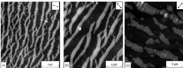
Figure 1. AFM image of the PET film with a gold coating ((a) 3 nm, (b) 5 nm, (c) 30 nm) stretched by 50% at 20°C via neck.
